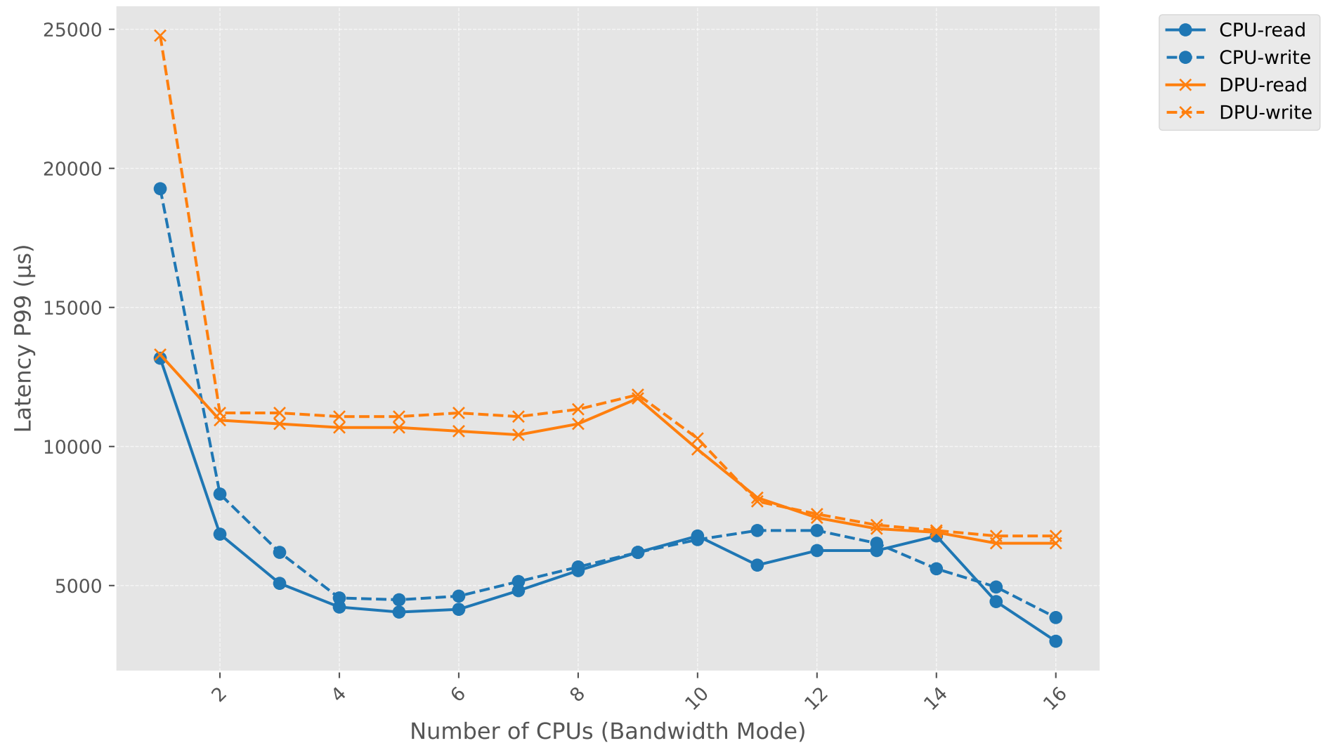
Latency P99 vs Number of CPUs (Bandwidth Mode)
